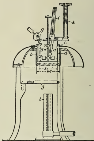
FIG. 182.—Pensky-Martens Closed Flash-point Tester.
